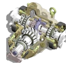
Final central reduction gears
